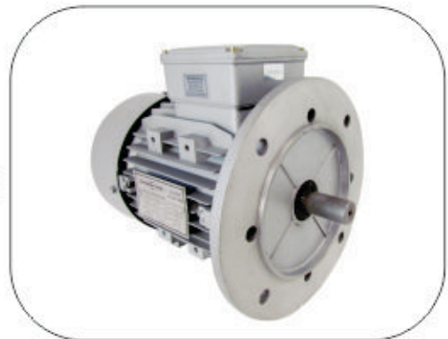
B5 Mounting
